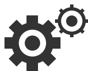
INTEGRATION API
