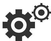
INTEGRATION API
